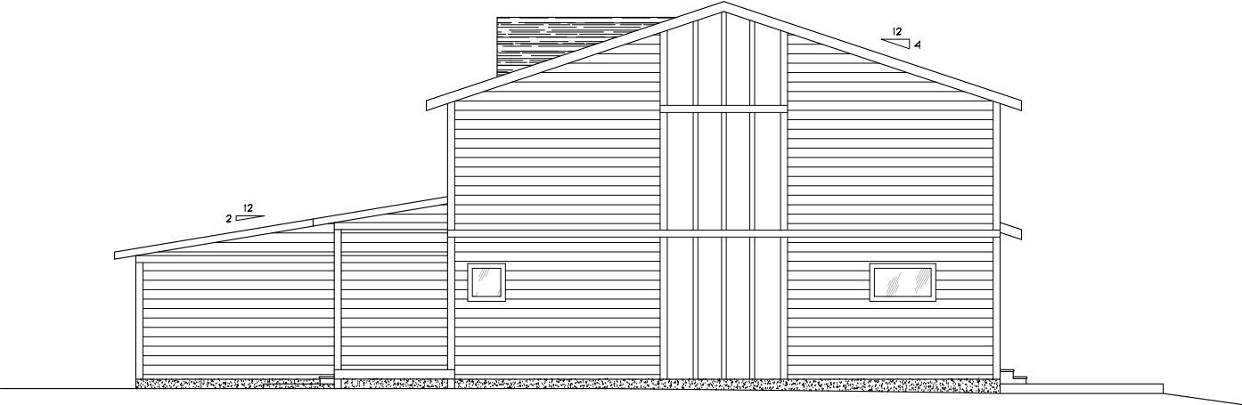
WEST ELEVATION
