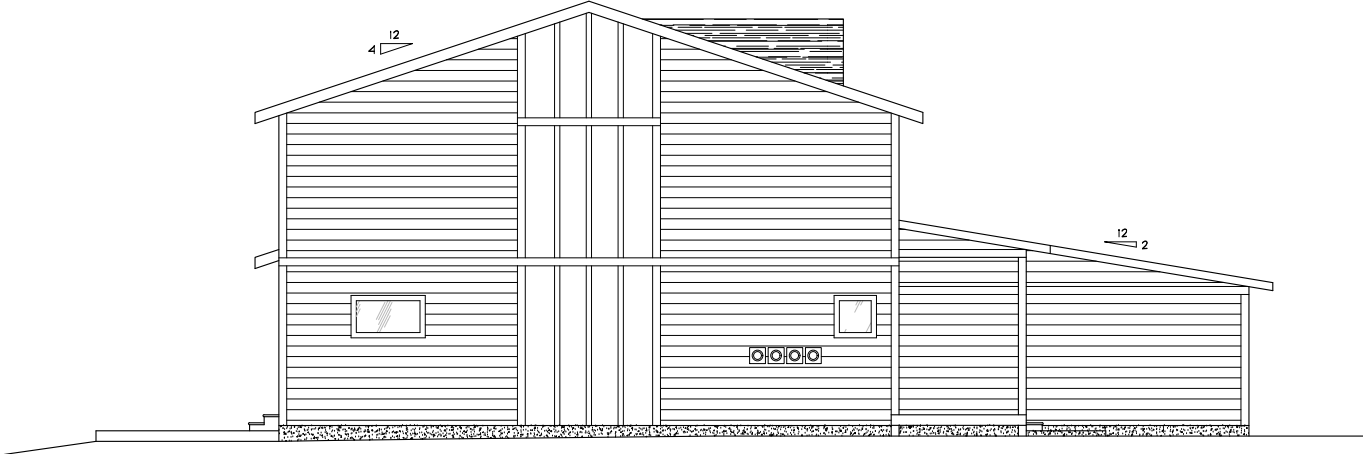
EAST ELEVATION
