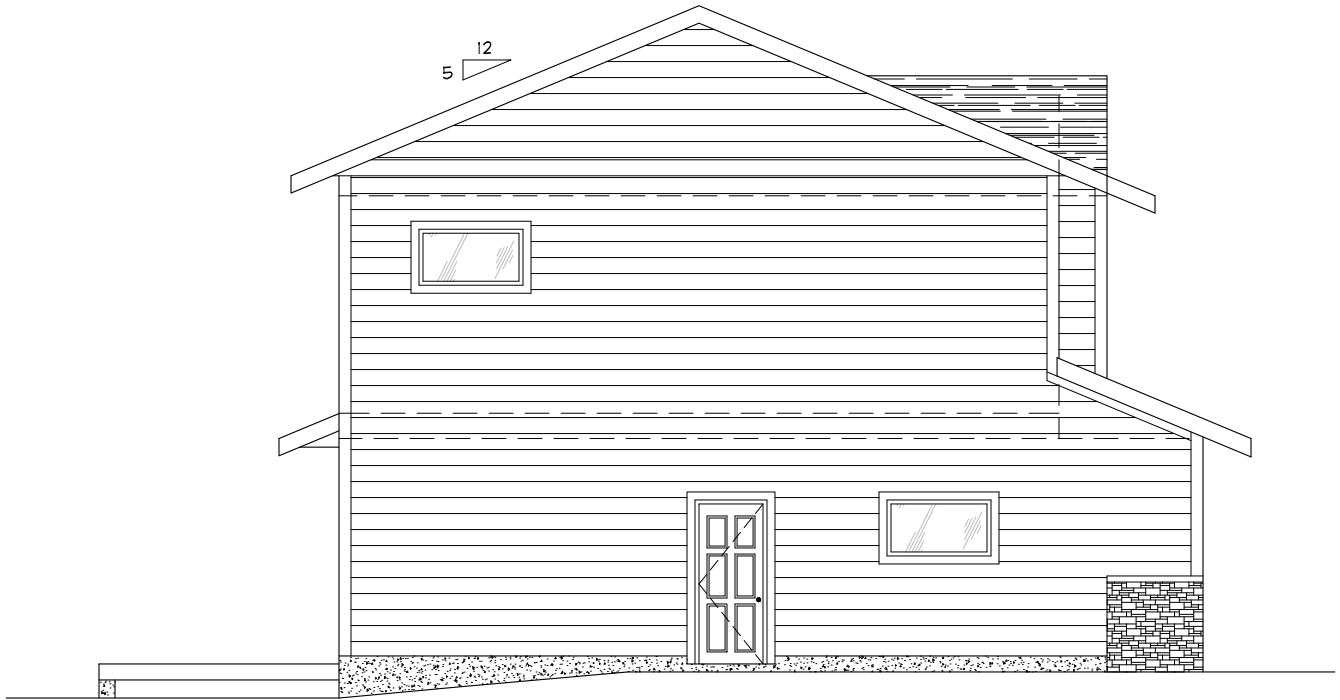
NORTH ELEVATION
