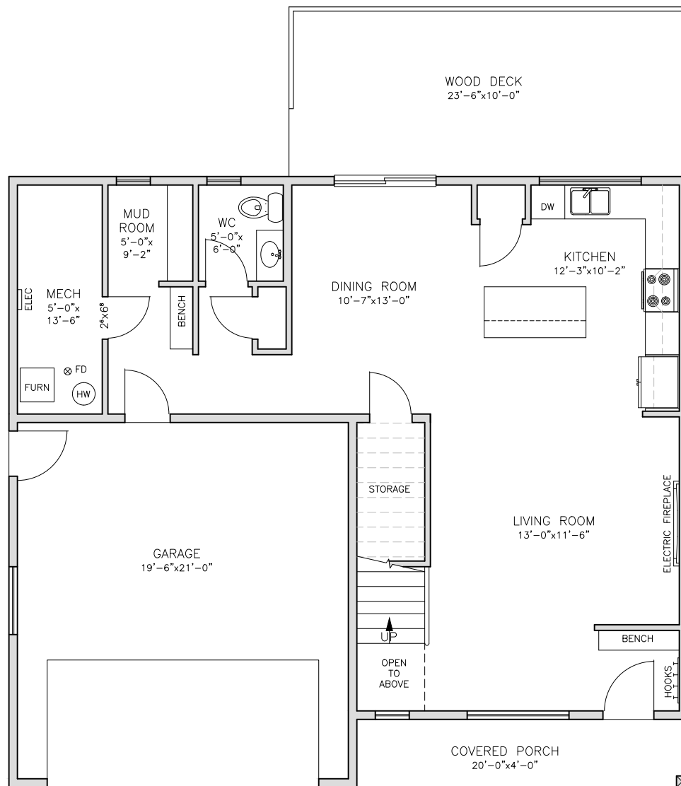
LOWER FLOOR PLAN 930 SQ FT
