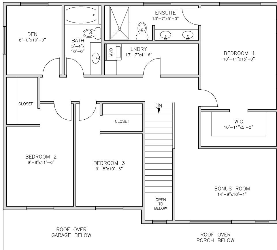
UPPER FLOOR PLAN 1240 SQ FT
